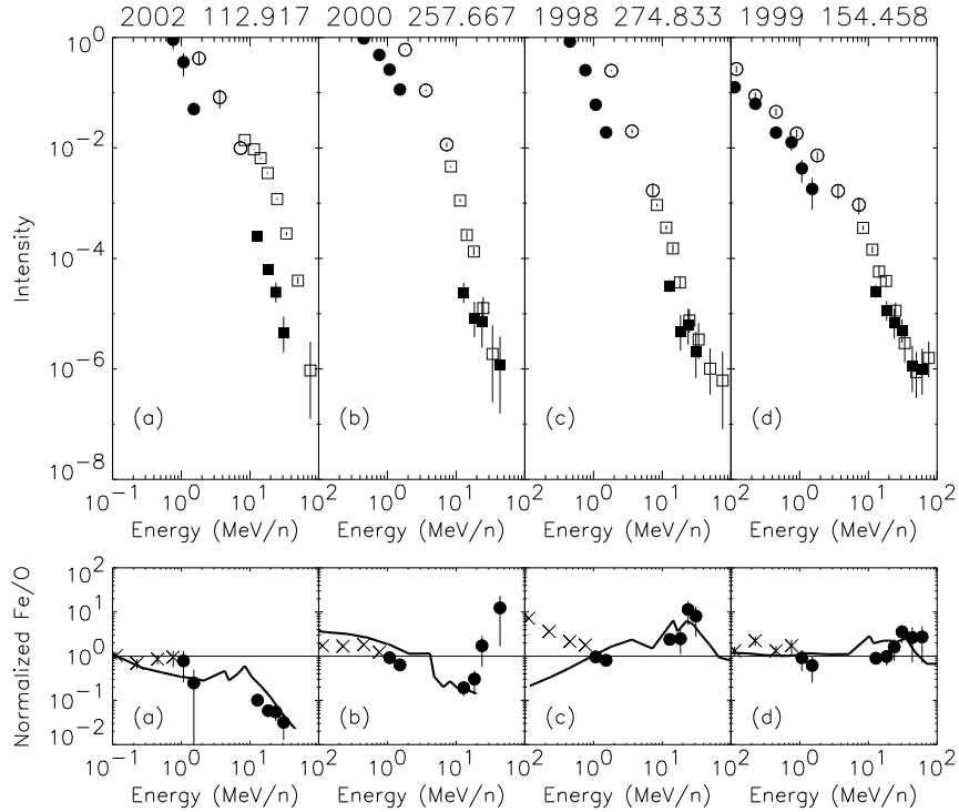
Fig. 2. Combined ULEIS (circles) and SIS (squares) oxygen (open symbols) and iron (closed symbols) spectra for 4 events (top panels). In the bottom panels filled circles indicate the Fe/O data used in the fit (normalized to the 1 MeV/nuc value), crosses are the remaining Fe/O values, and the solid lines show the simulated results.
