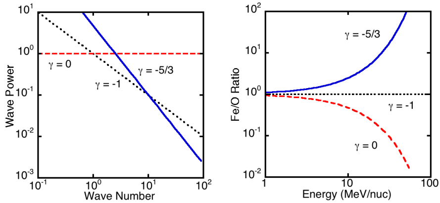
Fig. 1. Wave power spectra (left panel) in arbitrary units of different spectral indices and the energy dependence of the Fe/O ratio (right panel) predicted by the model of [1].
