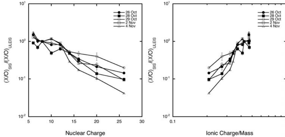
Figure 2. Abundances at 12-60 MeV/nucleon (from SIS, relative to oxygen) normalized by those at 0.77 MeV/nucleon (from ULEIS, relative to oxygen) versus nuclear charge (left) and charge/mass (right) of the elements for the 5 events.
