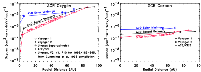
Figure 4. Intensity versus radial distance for ACR oxygen ( left ) and GCR carbon ( right ) from ACE ( circles ), Voyager 1 ( diamonds ), Voyager 2 ( squares ), and Ulysses ( stars ; see text) during the three time periods of interest. For solar minimum, values from an earlier study [4] ( triangles ) and without latitudinal gradient corrections ( crosses ) are also shown.
