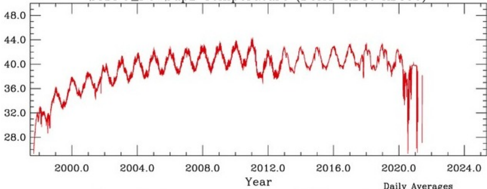
Sepica_IsoTank Temperature (DCM1-AD20 AD590)
