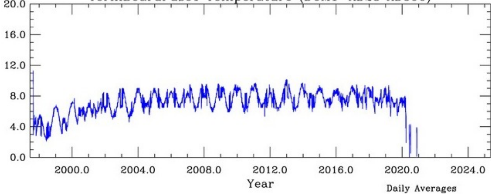
TermBoardFuse1 Temperature (DCM1-AD28 AD590)
