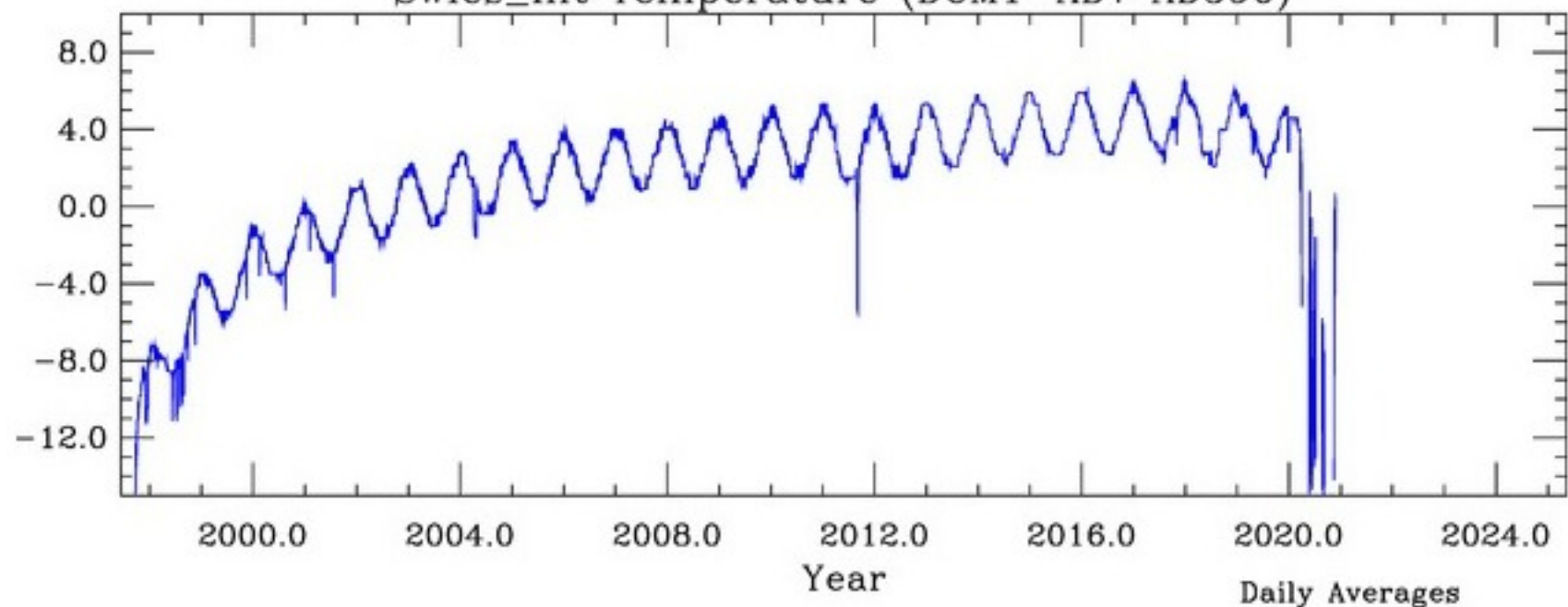
Swics_Int Temperature (DCM1-AD7 AD590)
