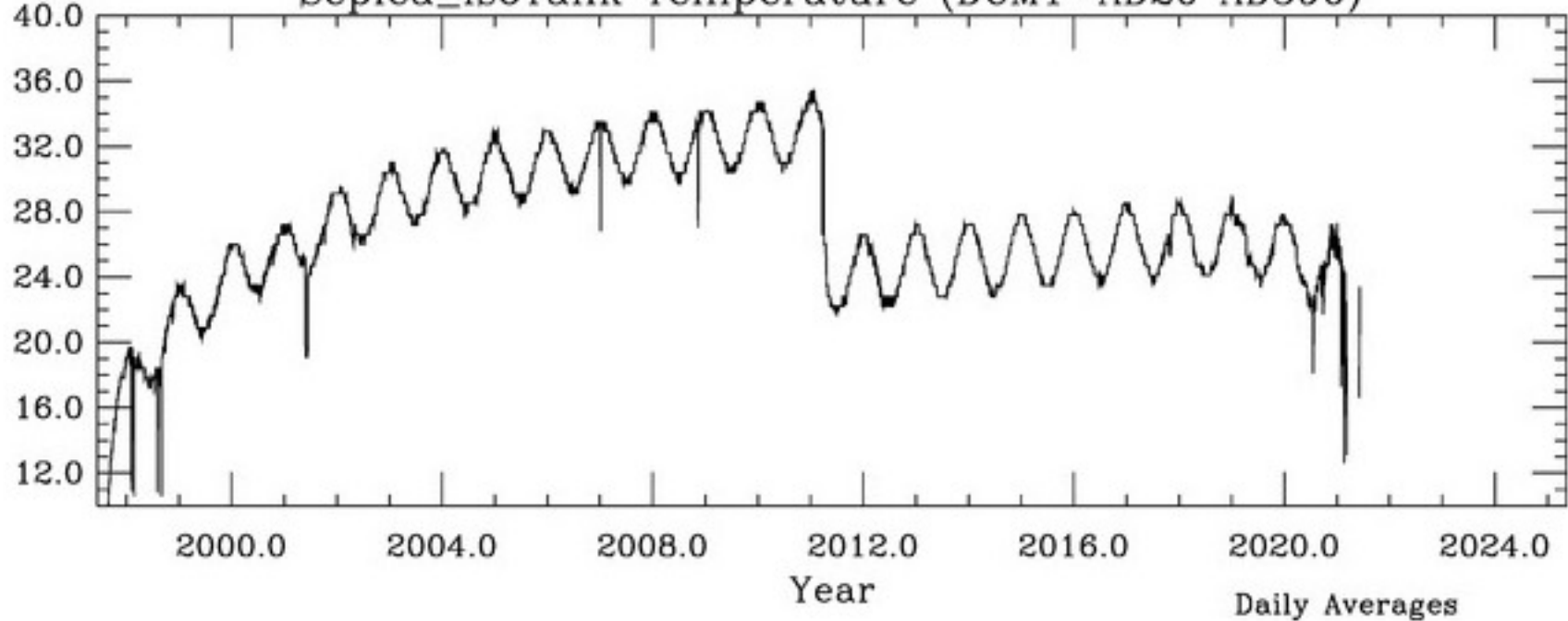
Sepica_IsoTank Temperature (DCM1-AD20 AD590)
