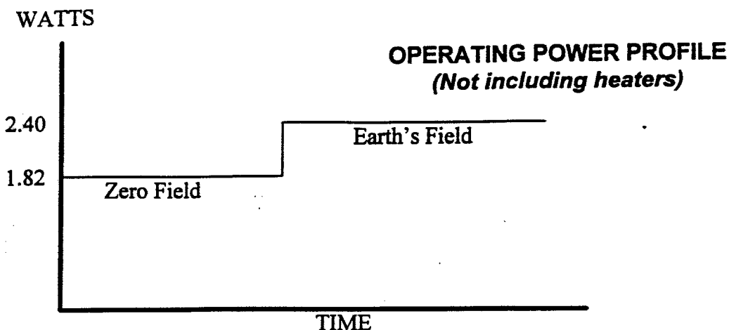
Figure 2.3.4-1 MAGNETOMETER Power Profile
