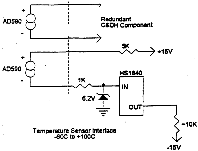
Figure 2.6.1.5.2-1 Temperature Sensor Interfaces
