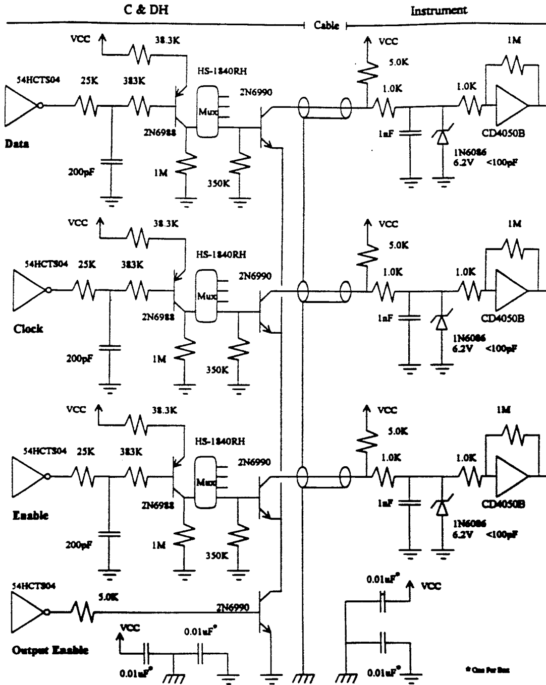
Figure 2.5.4.2.1-1 Data Command Interface
