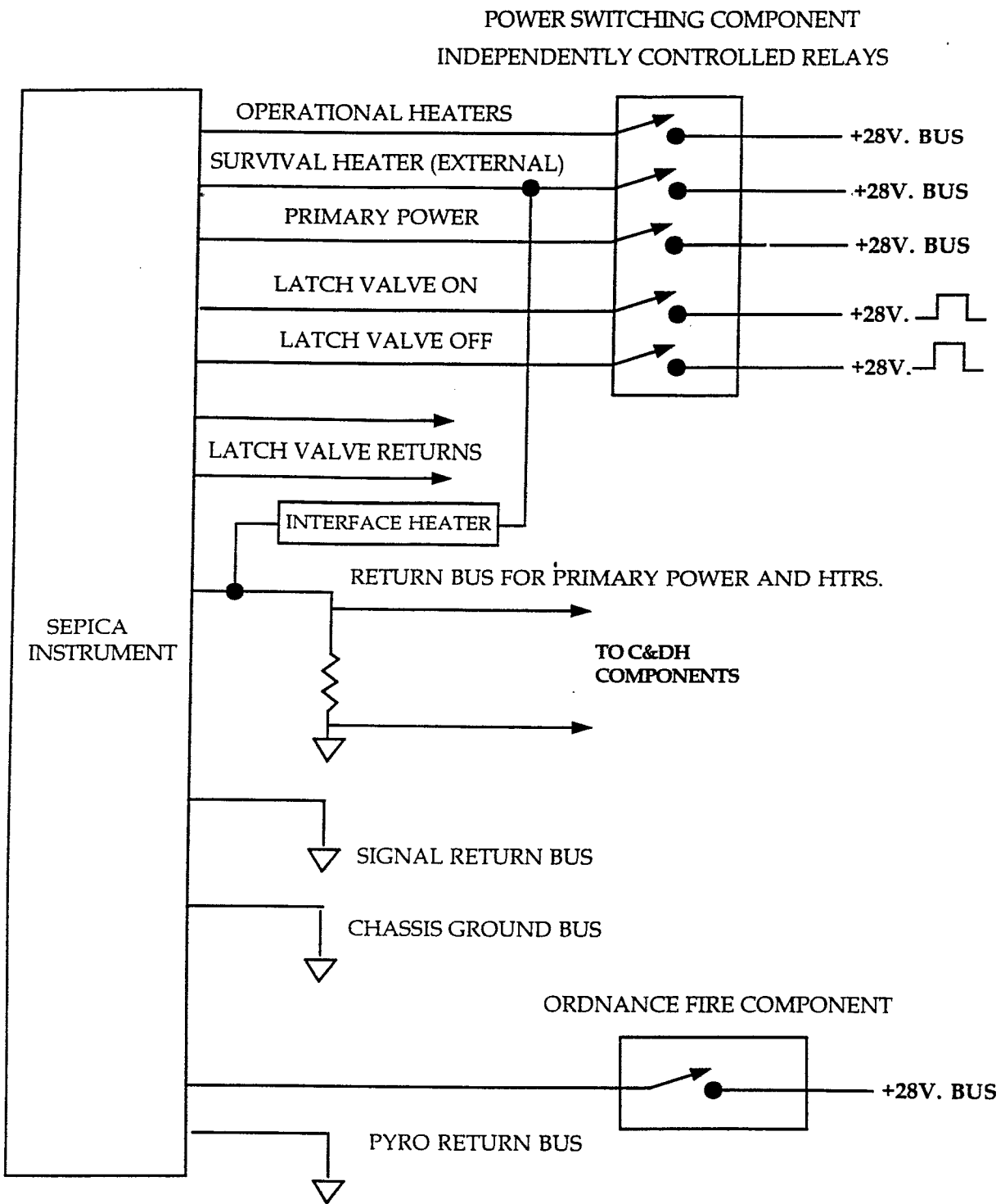
Figure 2.1-1 Functional Block Diagram of ACE Spacecraft/Instrument Electrical Interface (Cont.).
