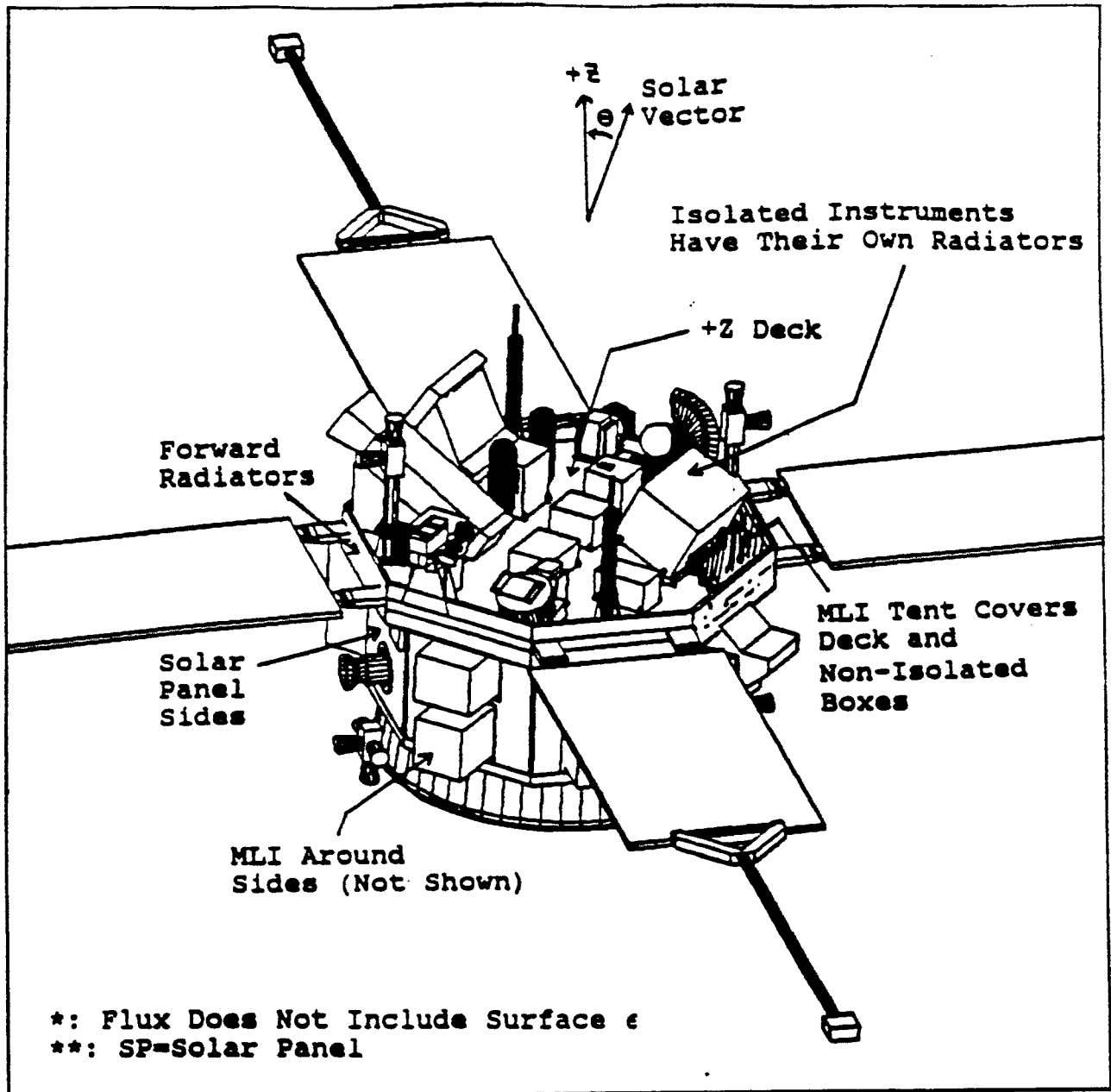
Figure 4.2-1 Preliminary Spacecraft Thermal Design Environment
