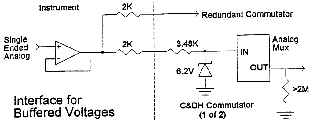
Figure 2.6.1.3.2-1 Single Ended Analog 0-5V Interface
