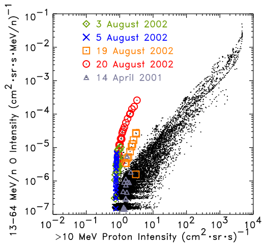
Fig. 2. Hourly ACE/SIS oxygen vs. proton rates, Aug 1997-Dec 2002.
