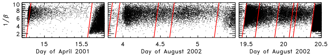
Fig. 3. SIS heavy ion velocity dispersion compared with X-ray flares ( see text ).
