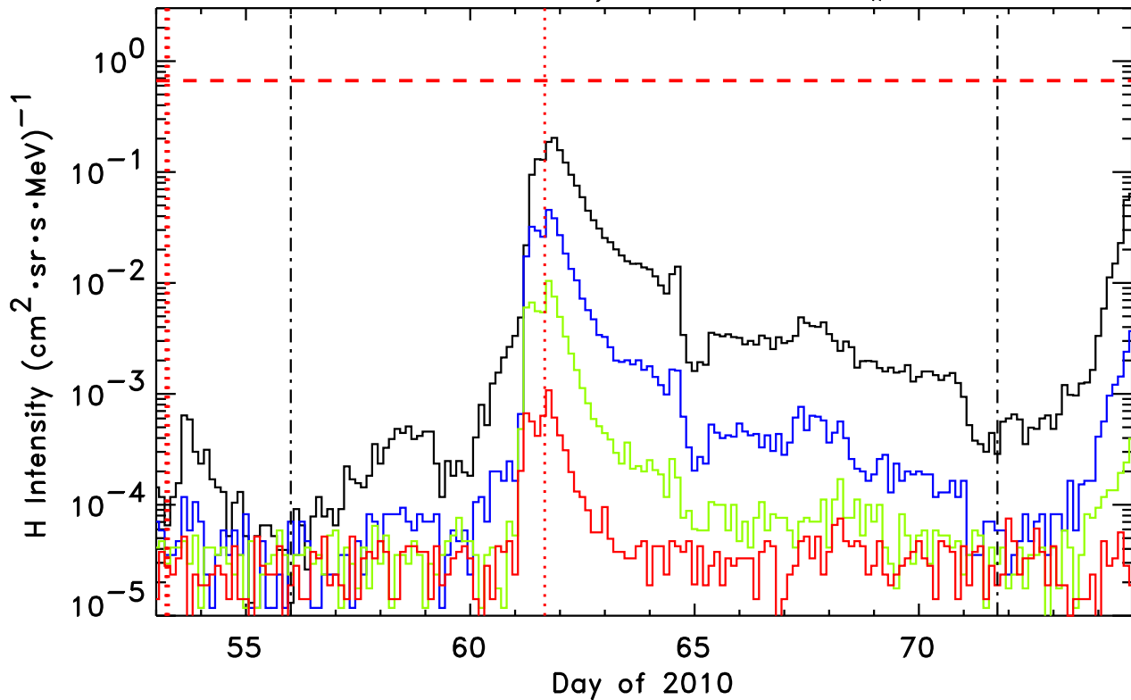
1.8-3.6, 4-6, 6-10, 10-15 MeV H STEREO-Ahead/LET He, Event #105
