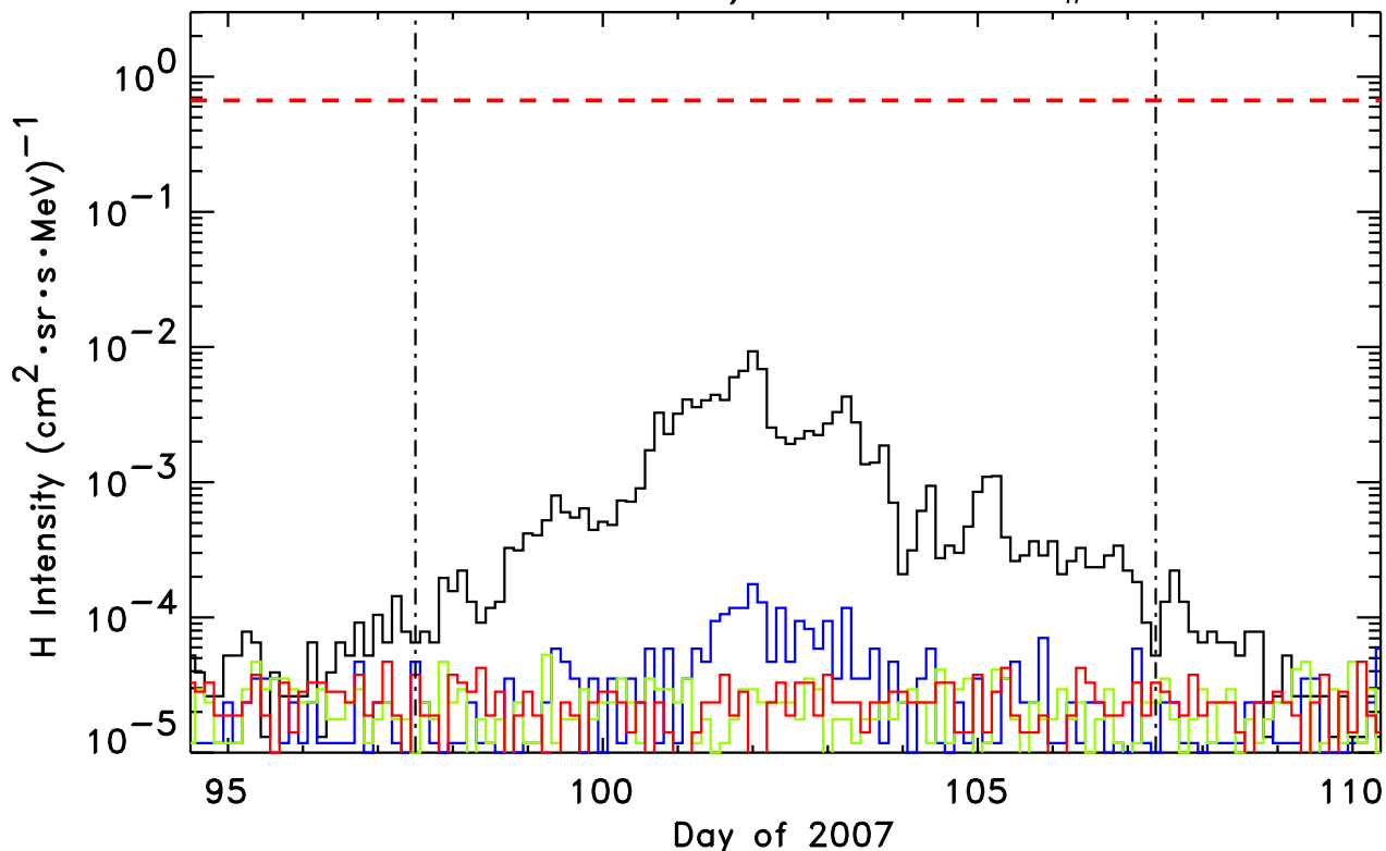
1.8-3.6, 4-6, 6-10, 10-15 MeV H STEREO-Ahead/LET He, Event # 14
