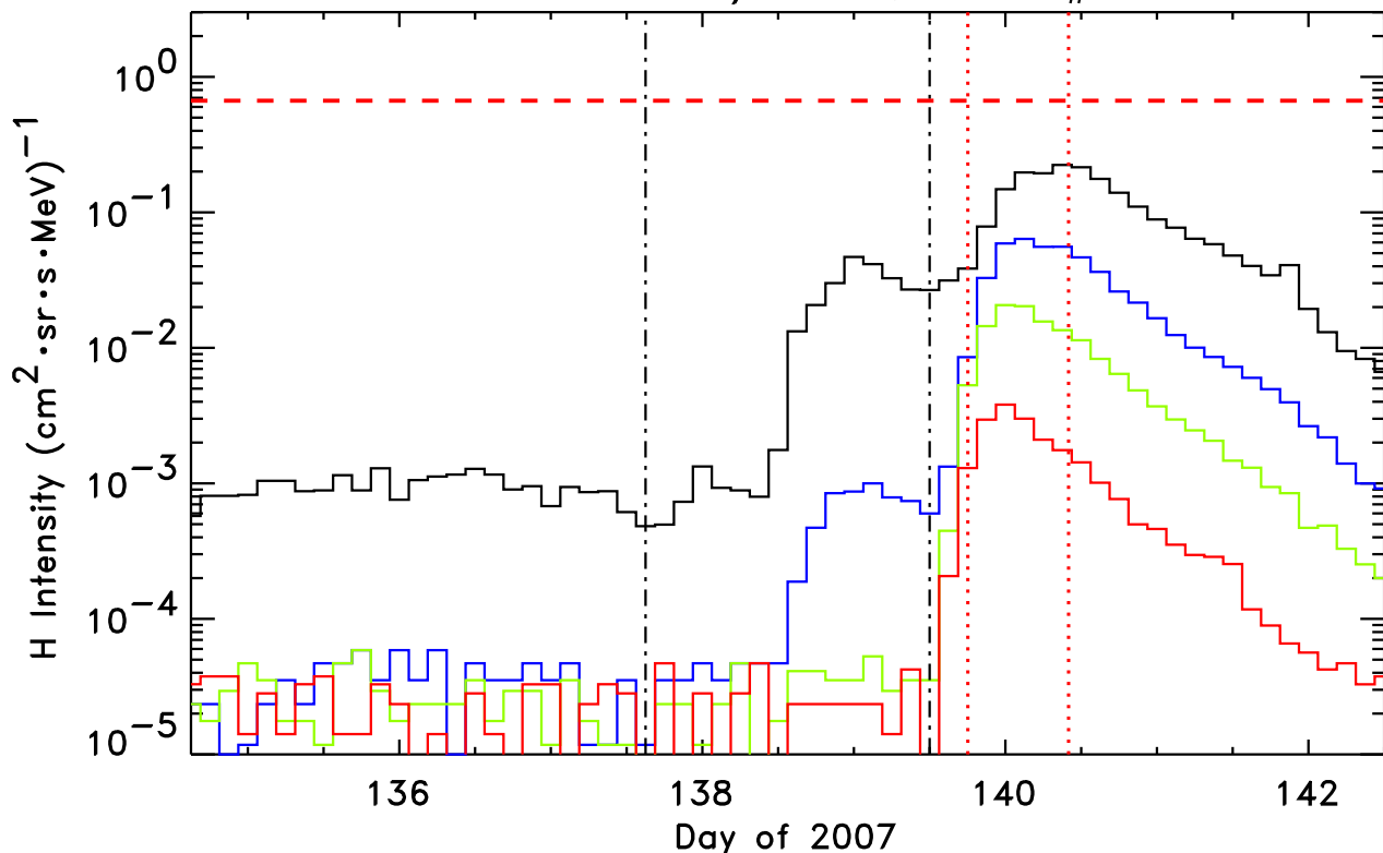
1.8-3.6, 4-6, 6-10, 10-15 MeV H STEREO-Ahead/LET He, Event # 16
