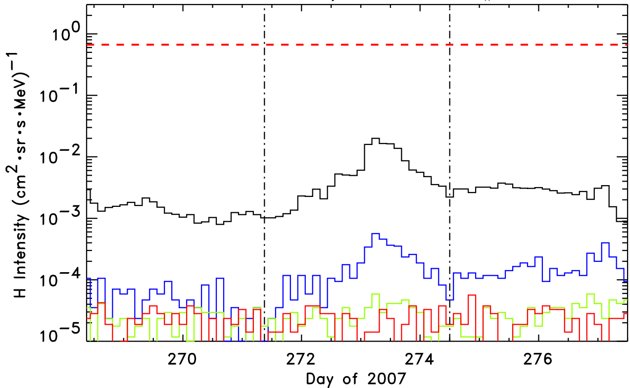
1.8-3.6, 4-6, 6-10, 10-15 MeV H STEREO-Ahead/LET He, Event # 30
