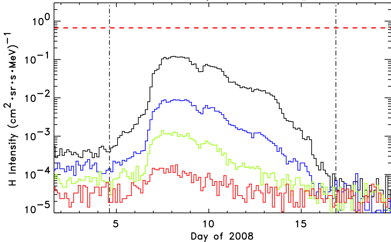
1.8-3.6, 4-6, 6-10, 10-15 MeV H STEREO-Ahead/LET He, Event # 40
