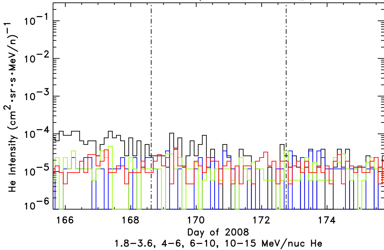
STEREO-Ahead/LET He, Event # 58
