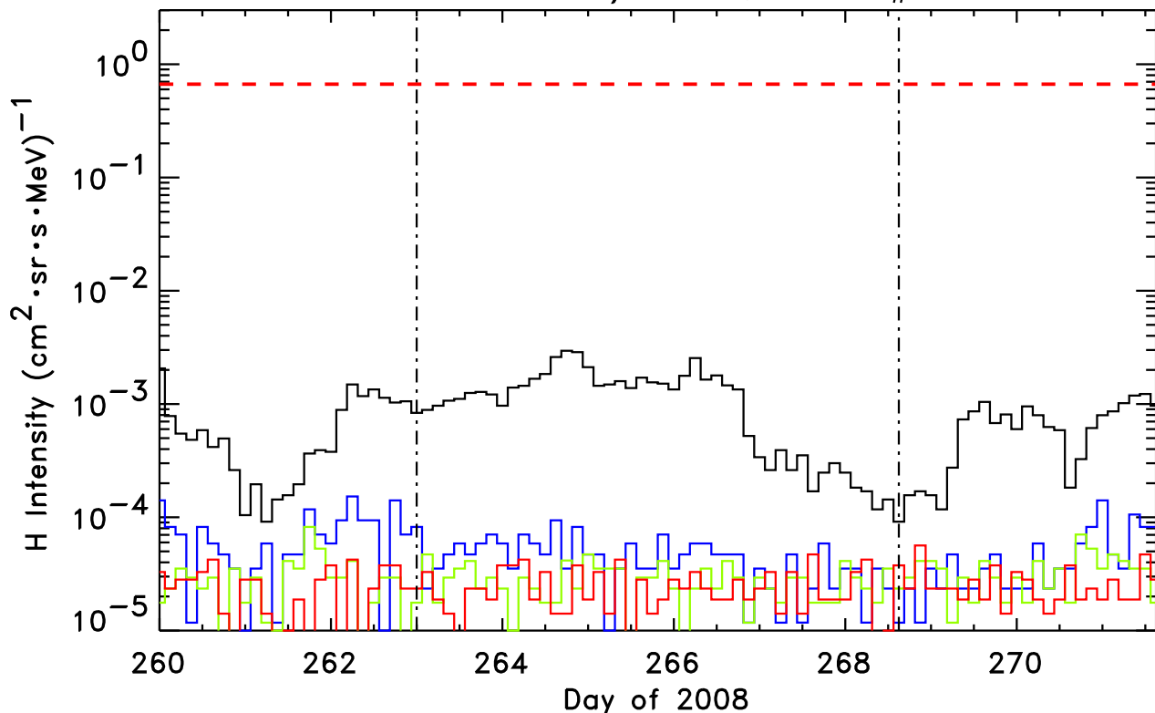
STEREO-Ahead/LET H, Event # 66
