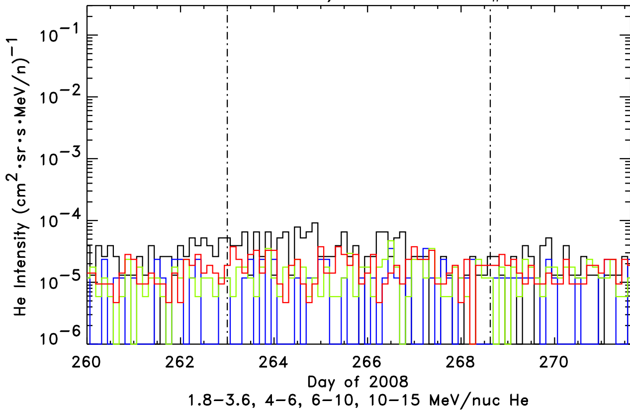
STEREO-Ahead/LET He, Event # 66
