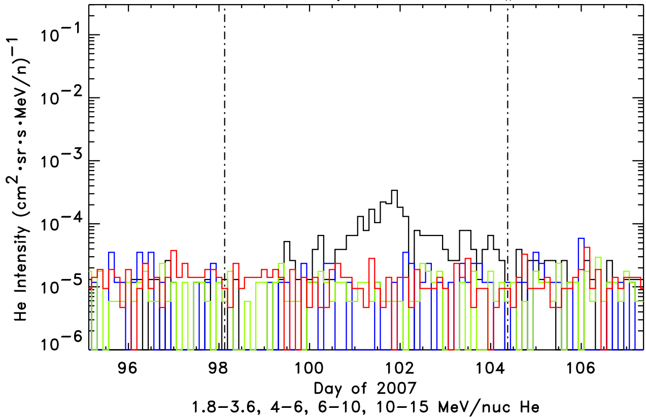
STEREO-Behind/LET He, Event # 12
