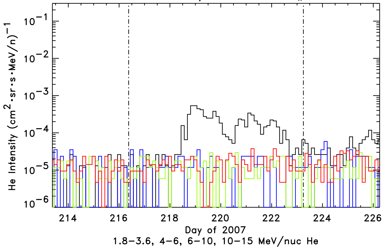
1.8-3.6, 4-6, 6-10, 10-15 MeV H STEREO-Behind/LET He, Event # 24
