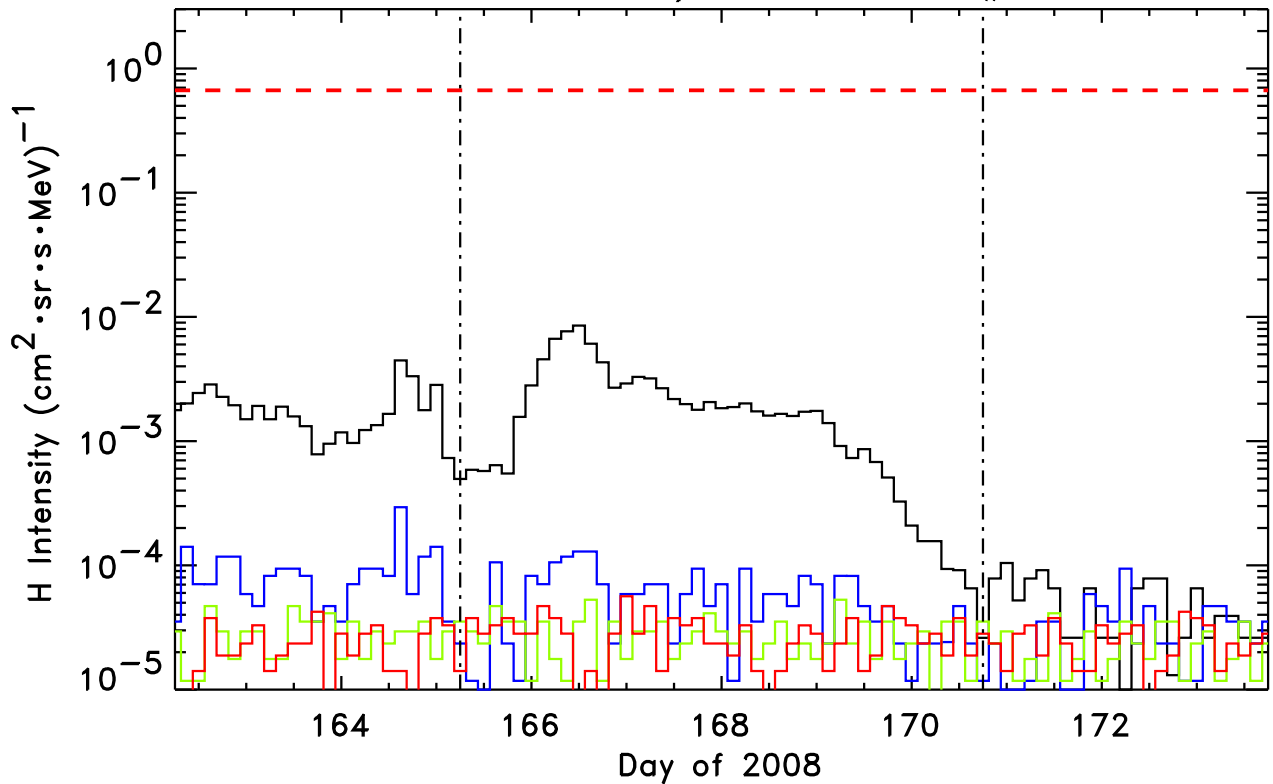
STEREO-Behind/LET H, Event # 59
