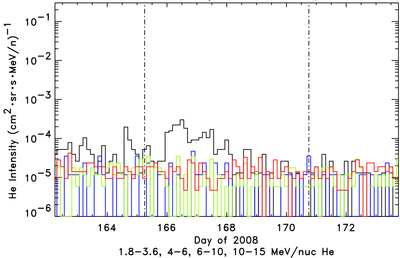
STEREO-Behind/LET He, Event # 59
