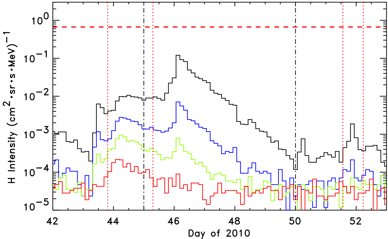
1.8-3.6, 4-6, 6-10, 10-15 MeV H STEREO-Ahead/LET He, Event #102
