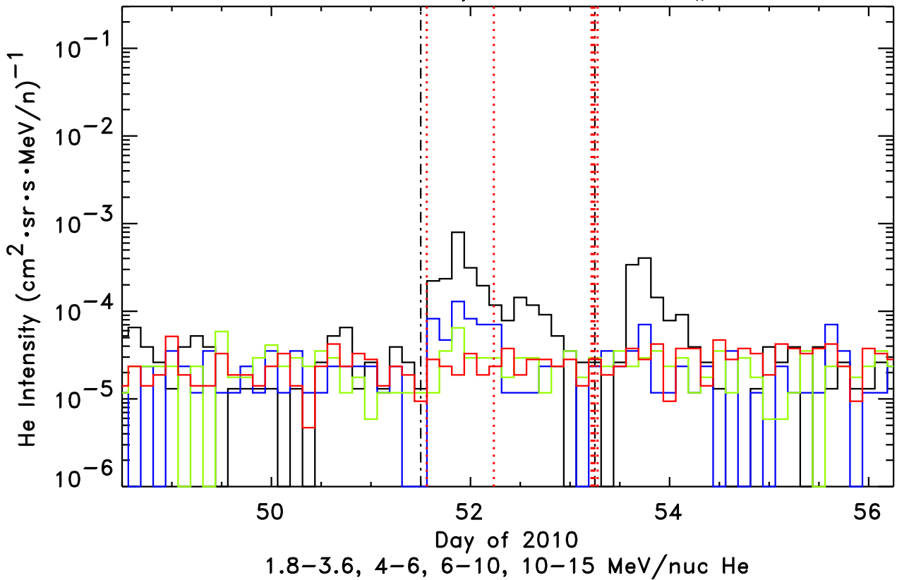
1.8-3.6, 4-6, 6-10, 10-15 MeV H STEREO-Ahead/LET He, Event #103
