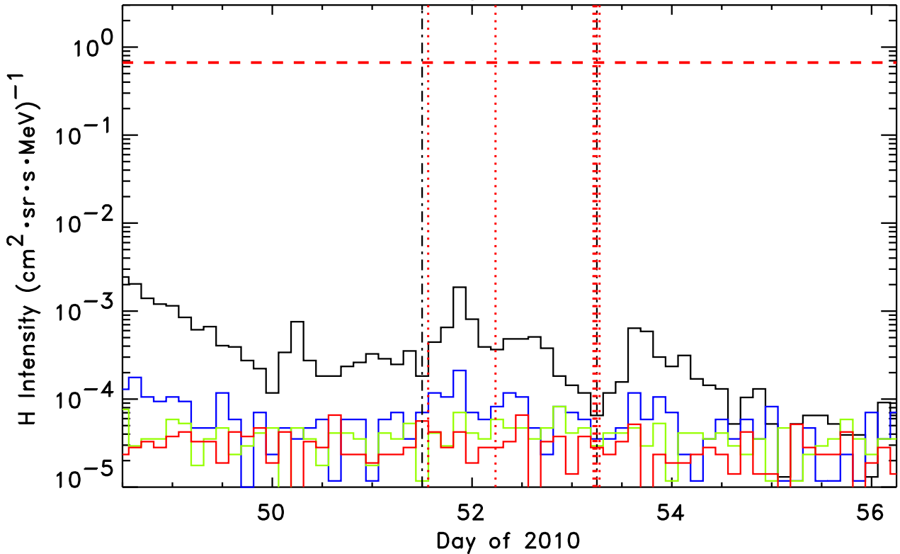
1.8-3.6, 4-6, 6-10, 10-15 MeV H STEREO-Ahead/LET He, Event #103
