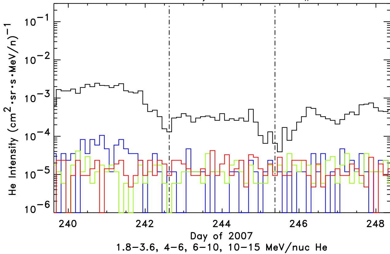
STEREO-Ahead/LET He, Event # 26
