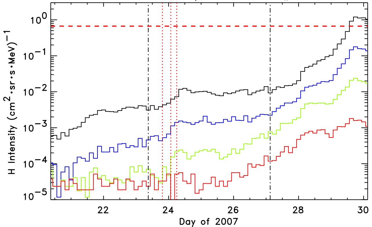
1.8-3.6, 4-6, 6-10, 10-15 MeV H STEREO-Ahead/LET He, Event # 4
