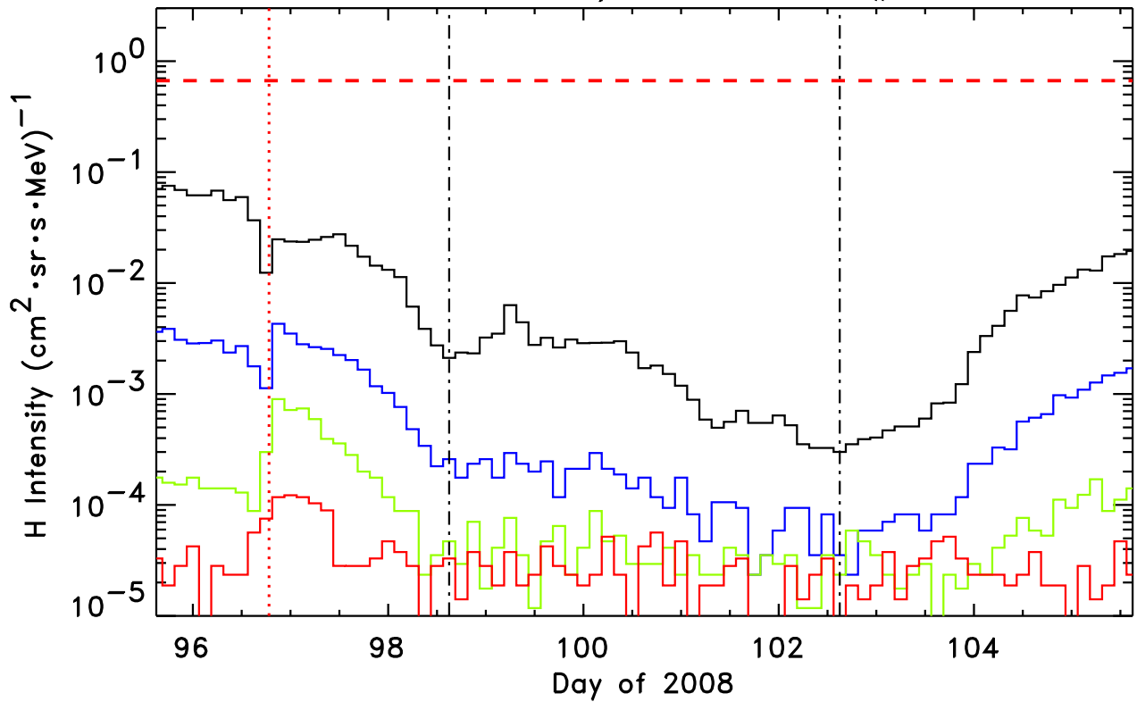
1.8-3.6, 4-6, 6-10, 10-15 MeV H STEREO-Ahead/LET He, Event # 52
