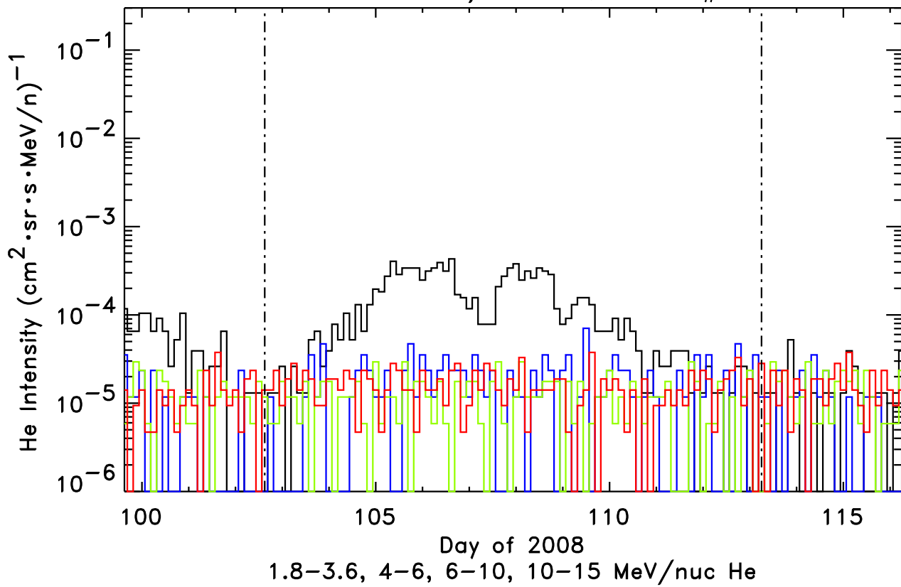
STEREO-Ahead/LET He, Event # 53
