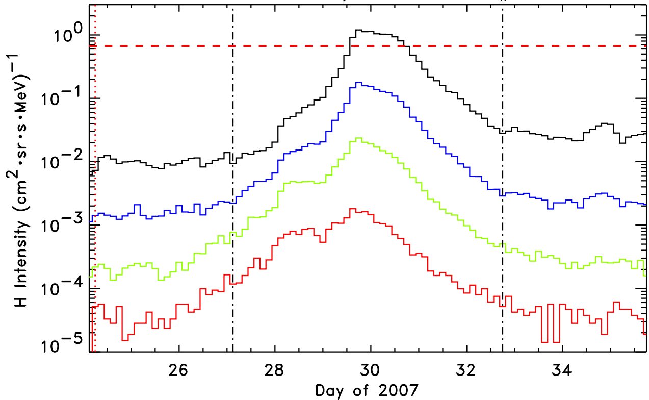
1.8-3.6, 4-6, 6-10, 10-15 MeV H STEREO-Ahead/LET He, Event # 5
