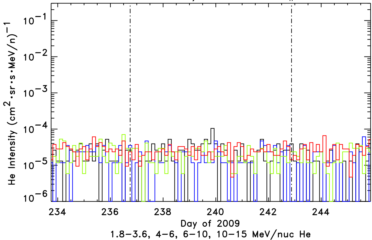
STEREO-Ahead/LET He, Event # 84
