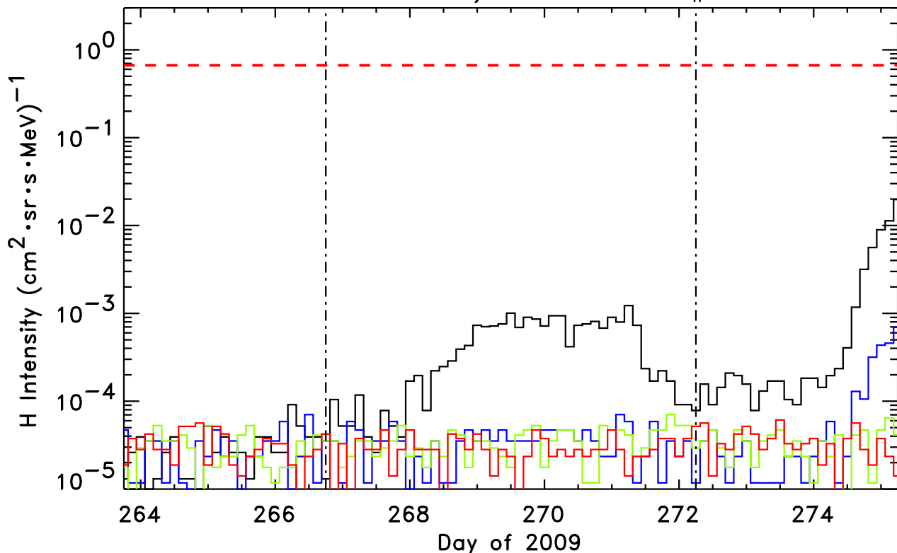
STEREO-Ahead/LET H, Event # 86
