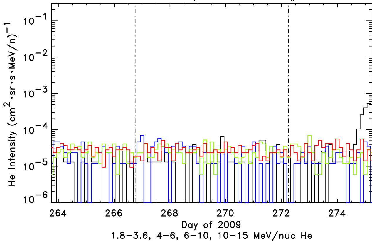
STEREO-Ahead/LET He, Event # 86
