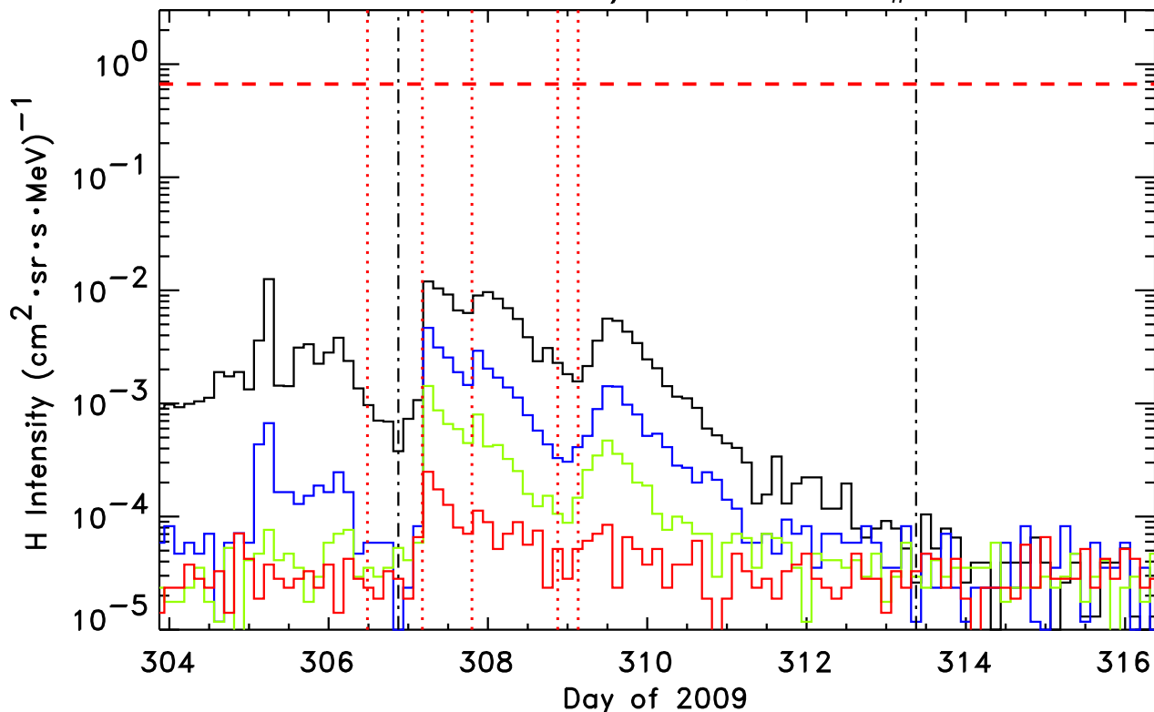
STEREO-Ahead/LET H, Event # 90
