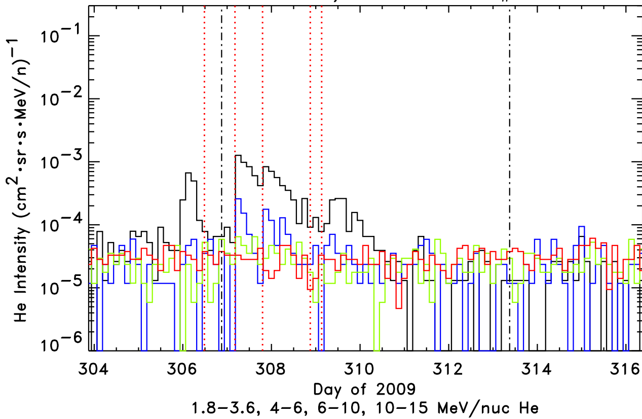
STEREO-Ahead/LET He, Event # 90
