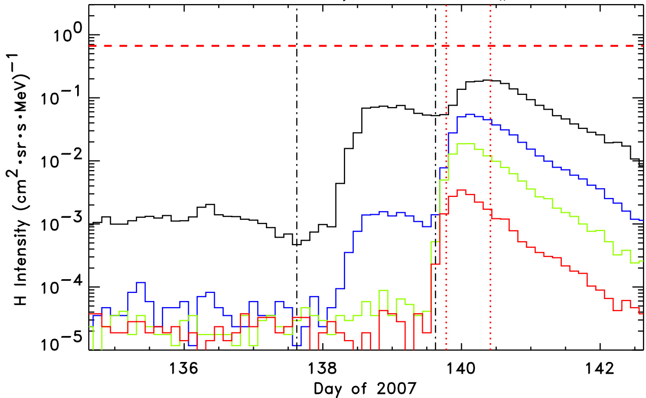
STEREO-Behind/LET H, Event # 15
