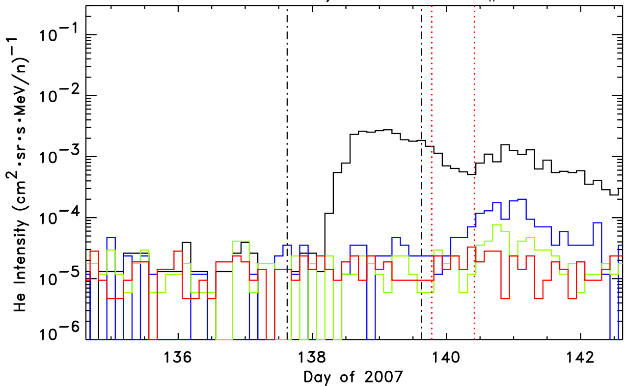
STEREO-Behind/LET He, Event # 15
