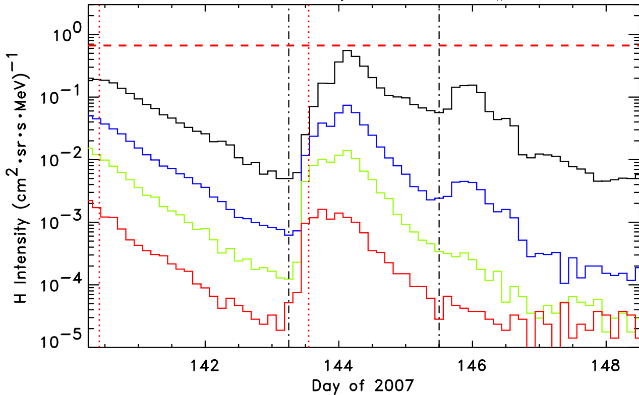
1.8-3.6, 4-6, 6-10, 10-15 MeV H STEREO-Behind/LET He, Event # 17
