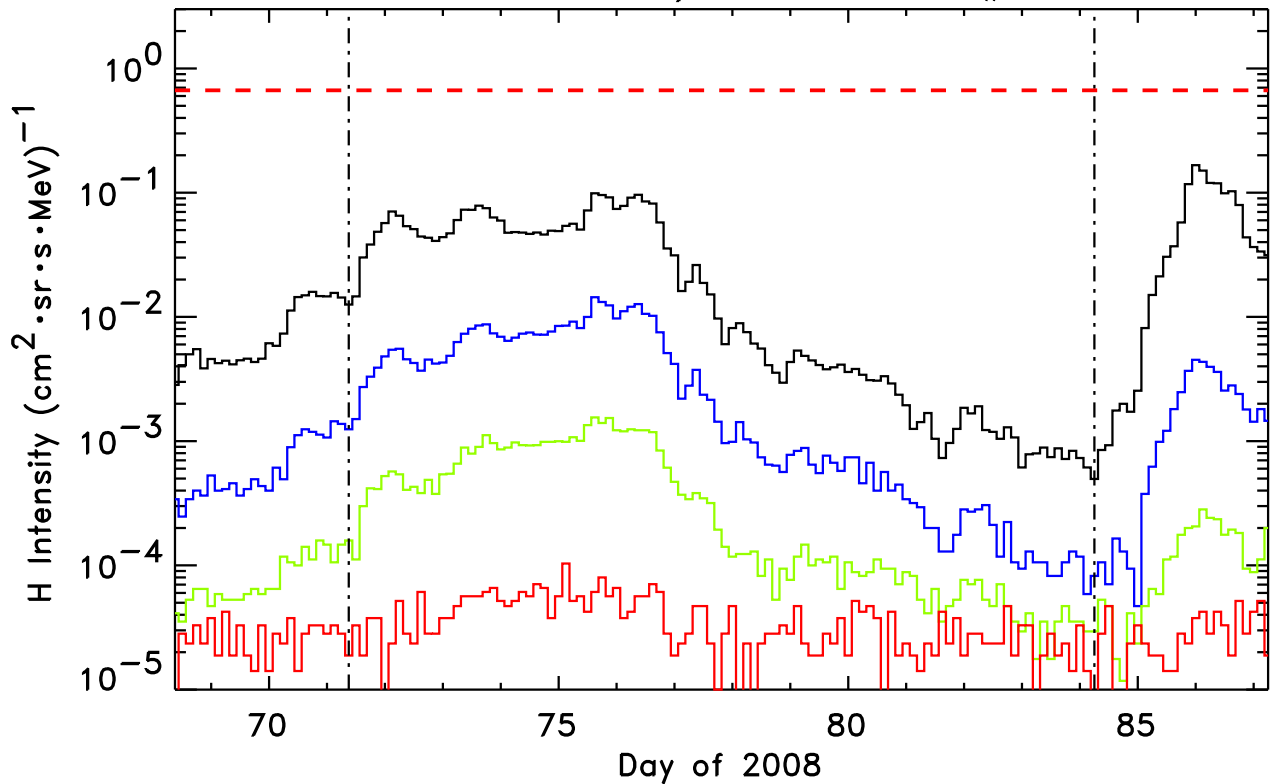
1.8-3.6, 4-6, 6-10, 10-15 MeV H STEREO-Behind/LET He, Event # 47
