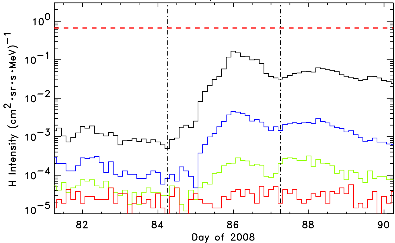
1.8-3.6, 4-6, 6-10, 10-15 MeV H STEREO-Behind/LET He, Event # 48
