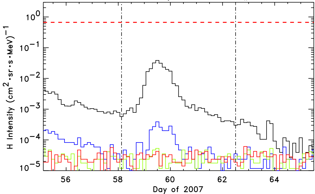
1.8-3.6, 4-6, 6-10, 10-15 MeV H STEREO-Behind/LET He, Event # 8
