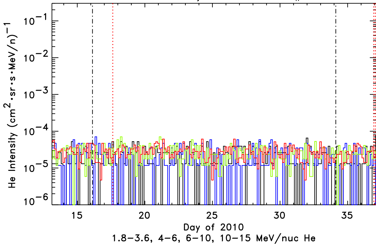
STEREO-Behind/LET He, Event # 90
