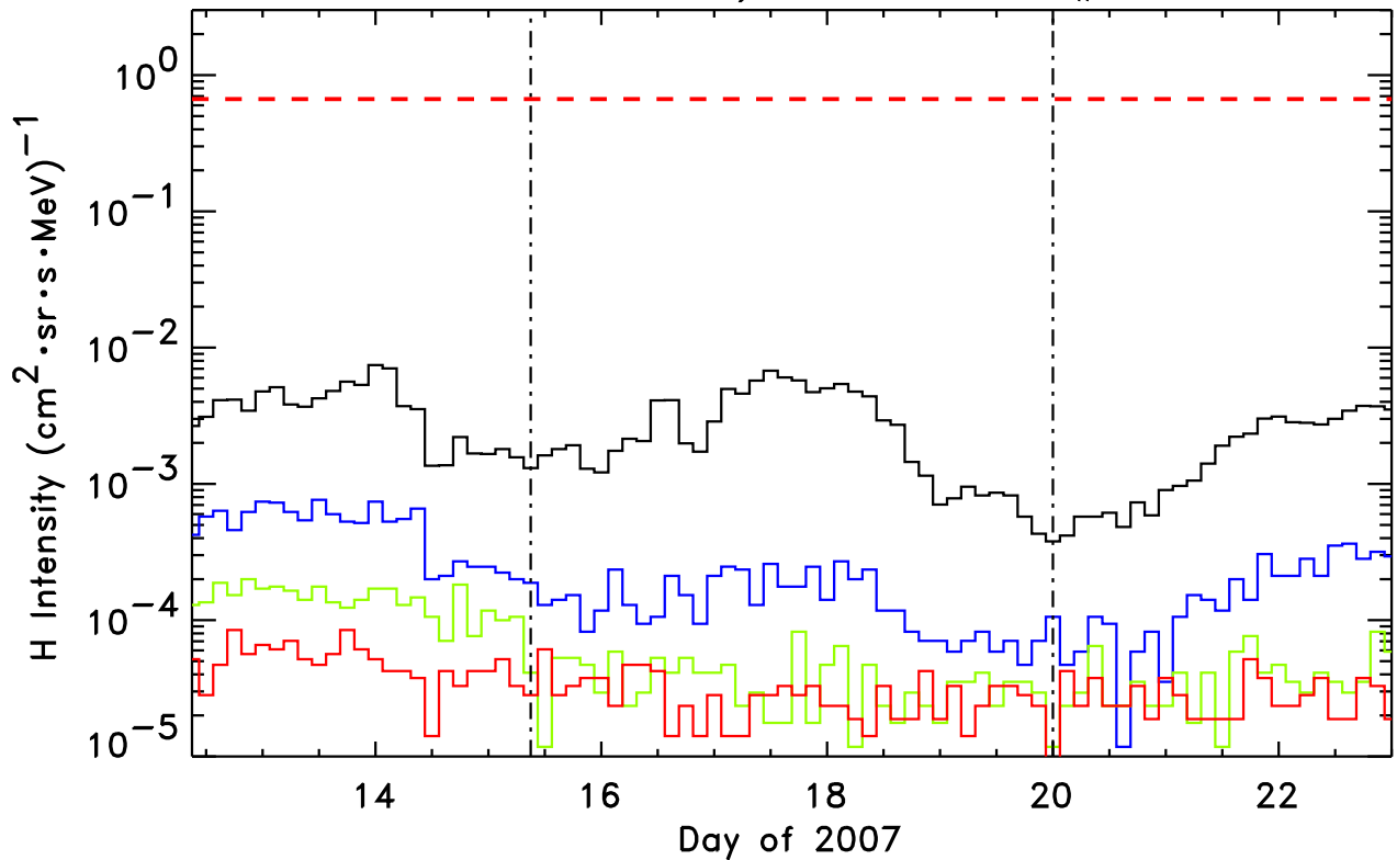
1.8-3.6, 4-6, 6-10, 10-15 MeV H STEREO-Ahead/LET He, Event # 2
