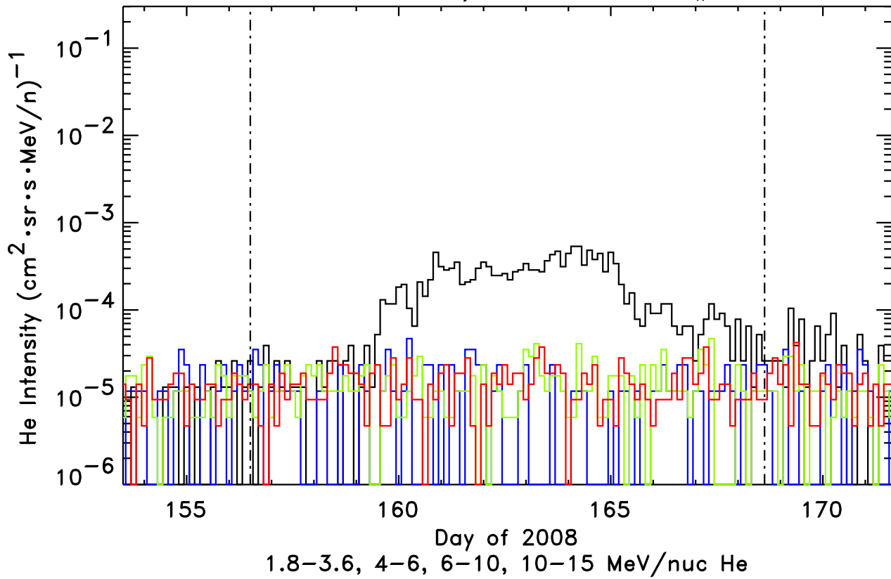
STEREO-Ahead/LET He, Event # 57
