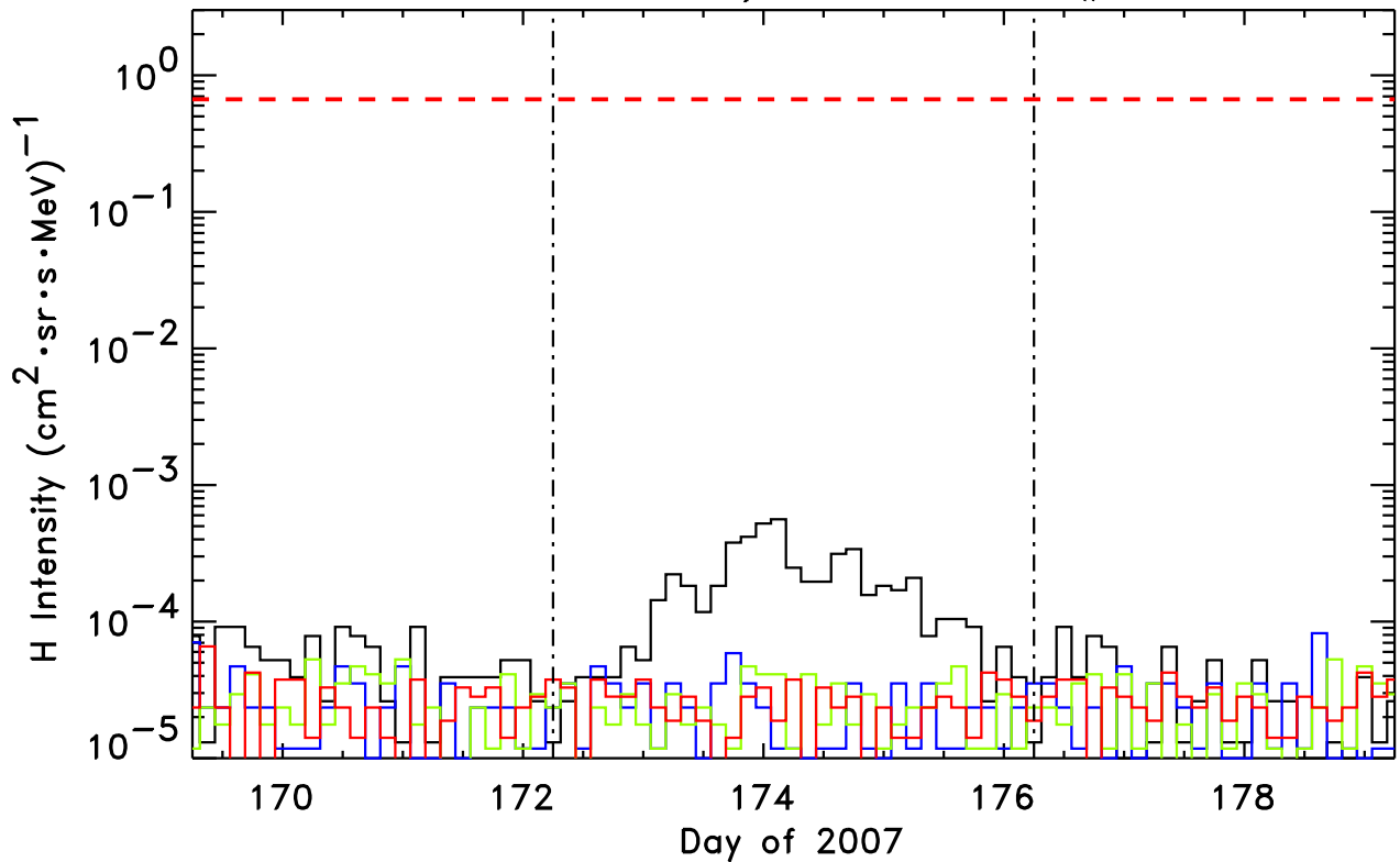
1.8-3.6, 4-6, 6-10, 10-15 MeV H STEREO-Behind/LET He, Event # 20
