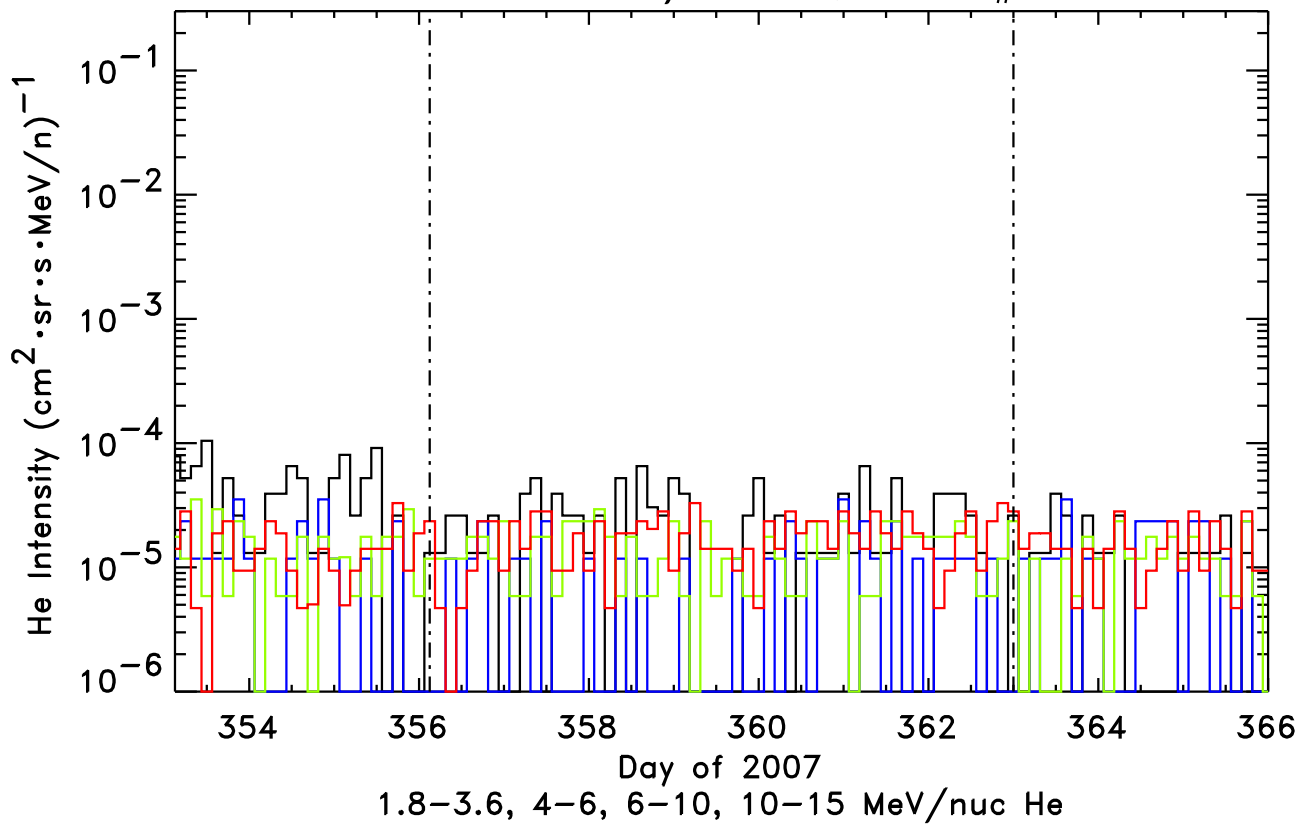
1.8-3.6, 4-6, 6-10, 10-15 MeV H STEREO-Behind/LET He, Event # 39
