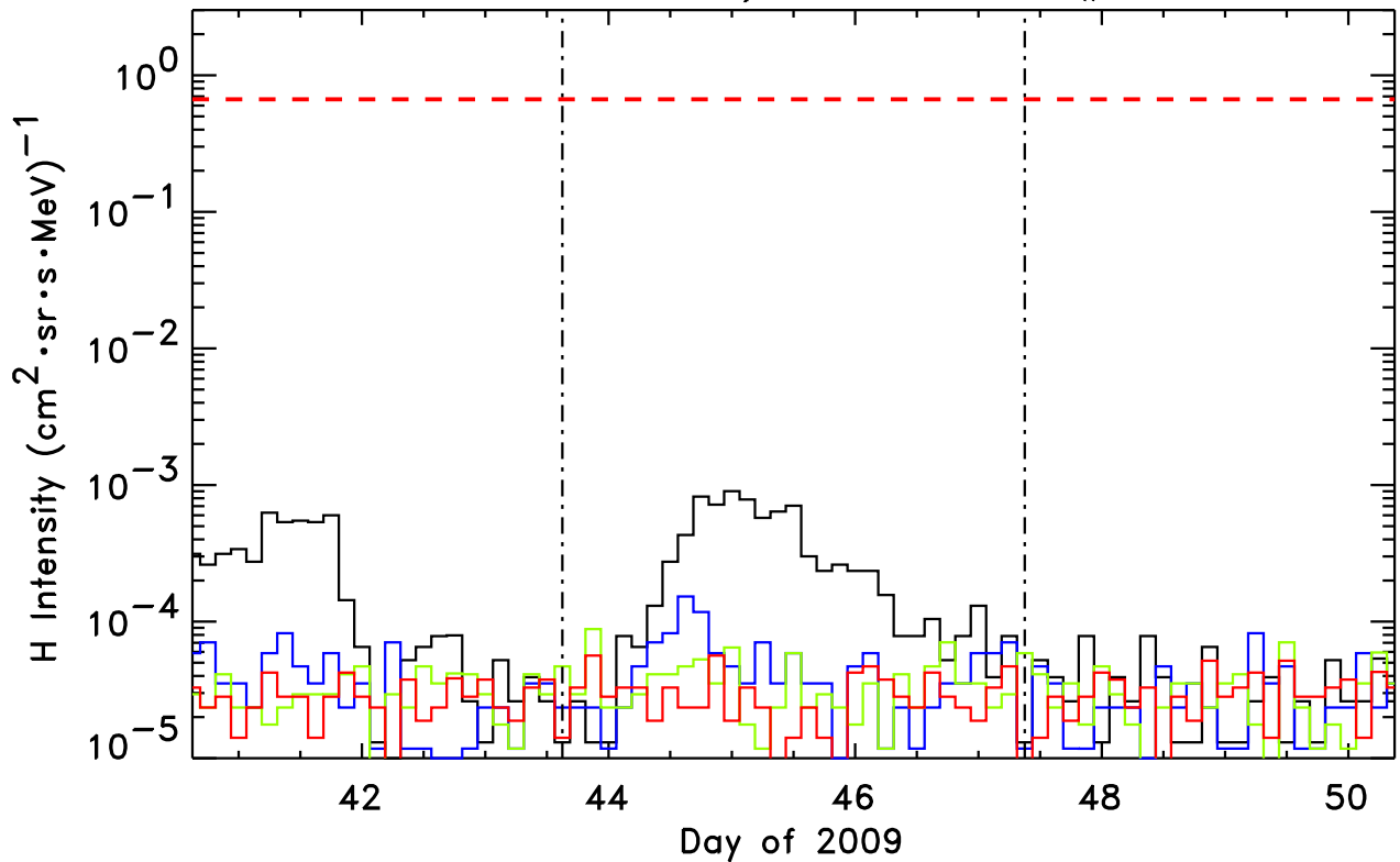
1.8-3.6, 4-6, 6-10, 10-15 MeV H STEREO-Behind/LET He, Event # 79
