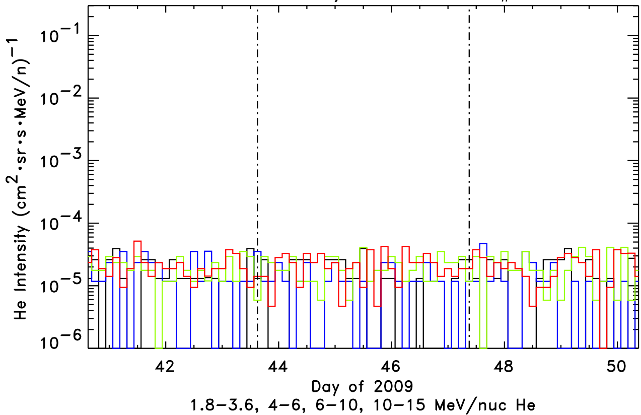
1.8-3.6, 4-6, 6-10, 10-15 MeV H STEREO-Behind/LET He, Event # 79
