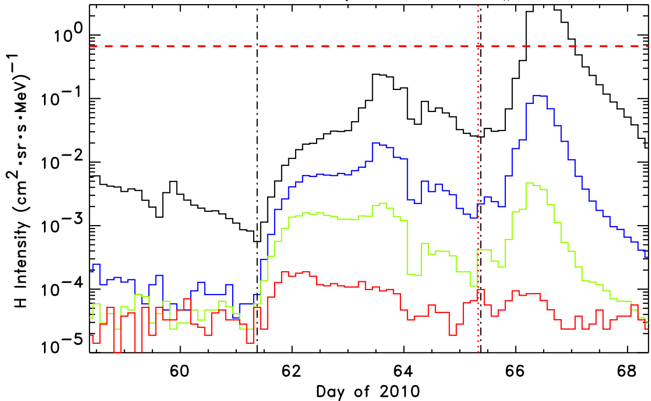
1.8-3.6, 4-6, 6-10, 10-15 MeV H STEREO-Behind/LET He, Event # 95
