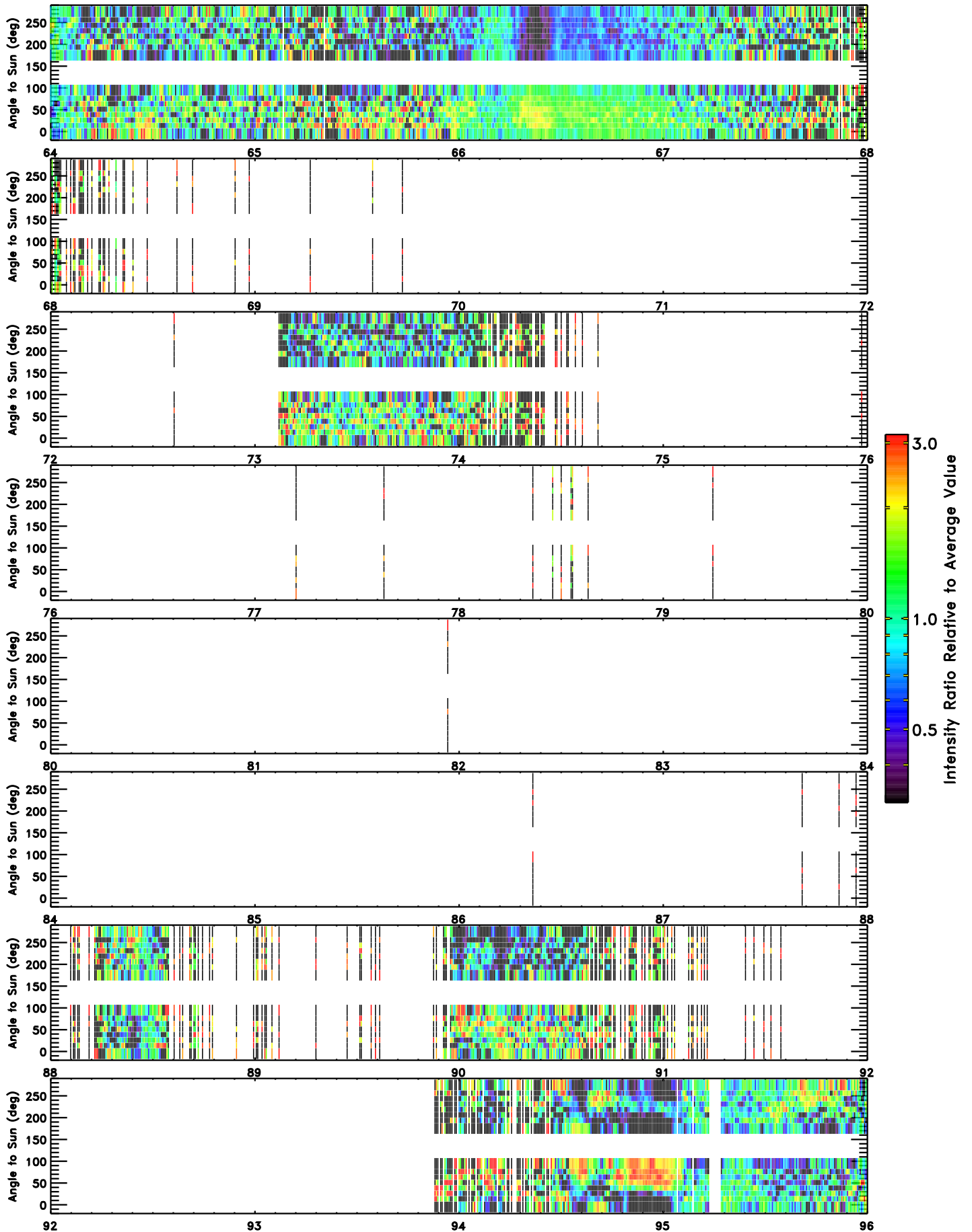
Day of 2010 10-minute averages, 3-point smoothed, >2 counts/10 min period
