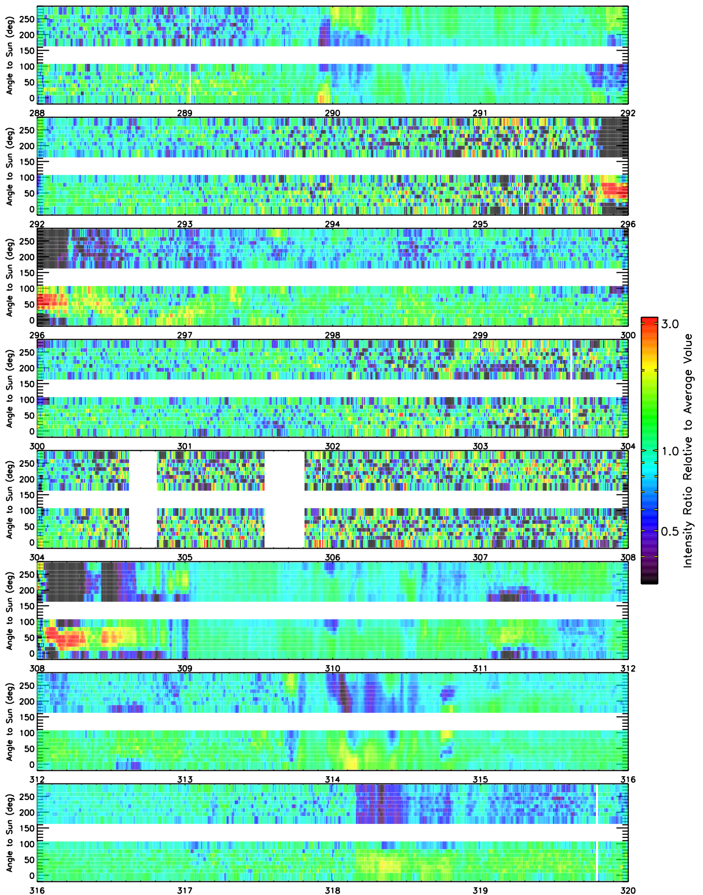
Day of 2011 10-minute averages, 3-point smoothed, >2 counts/10 min period
